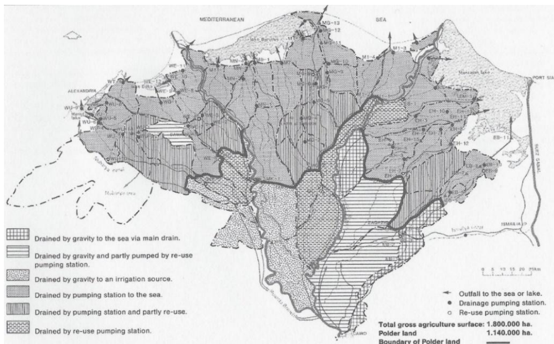
Figure 3. Polders in the Nile Delta and the drainage basins of the delta with their drainage system (Wolters et al. , 1986)
