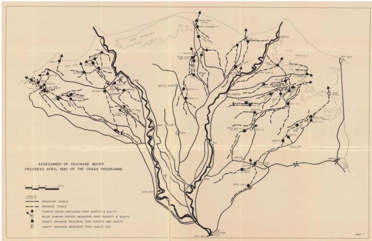
Figure 6. Drains in the Nile Delta – 1980
